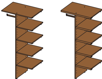
T partitioning | T partitioning with wide edge
