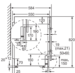
Detail Z
